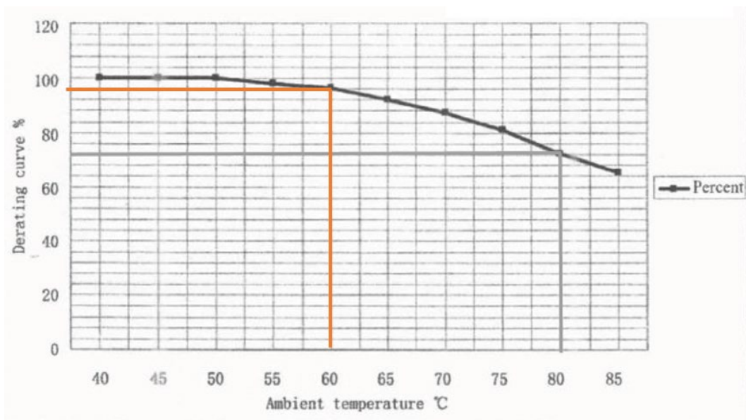
Figure 8.2 Example of temperature de-rating curve showing de-rating points at 60° and 80°
